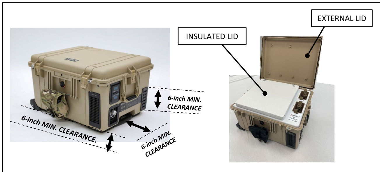
Figure 6: xFridge Setup
